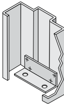
ONE PIECE WELDED BASED ANCHOR
